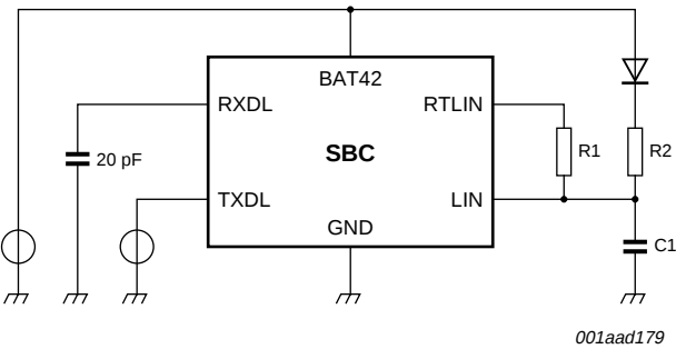
Fig 25. Timing test circuit for LIN transceiver
