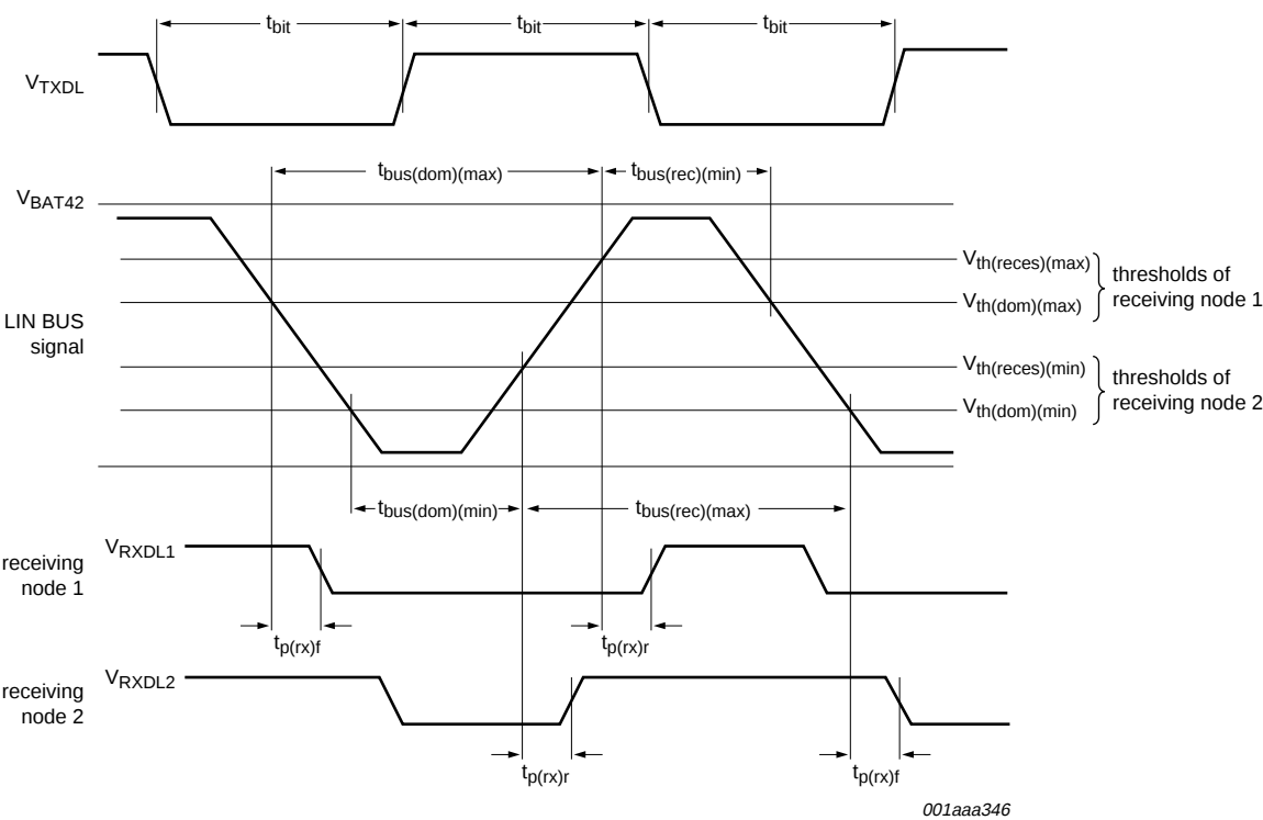
Fig 26. Timing diagram LIN transceiver
